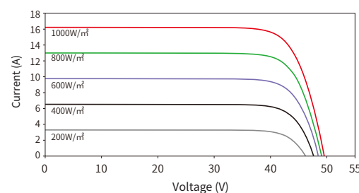
Current-Voltage Curves (VSP630DM 625W)
