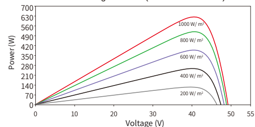
Power-Voltage Curves (VSP630DM 625W)
